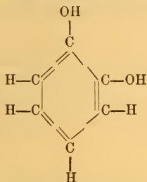
Pyrocatechin, oxyphenic acid, catechol.
